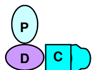
Cytosine (C)
