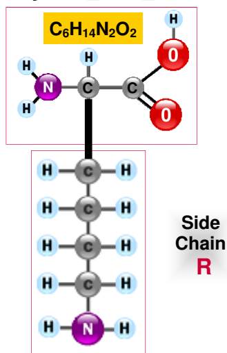
Lysine LYS_K
