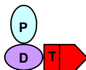
Thymine (T)
