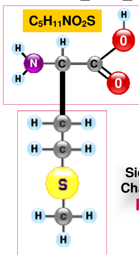
Methionine MET_M
